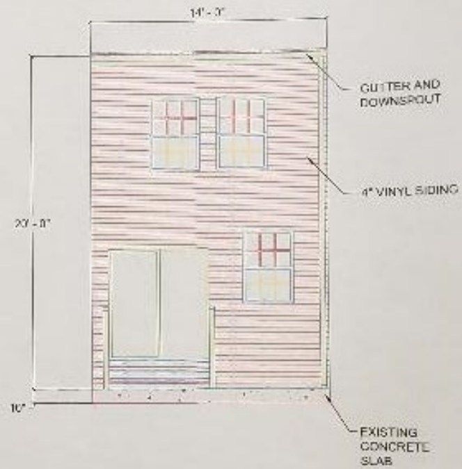
1 REAR ELEVATION Scale: 1/4"=1'-0"
