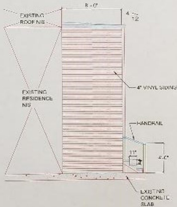
2 SIDE ELEVATION Scale: 1/4"=1'-0"
